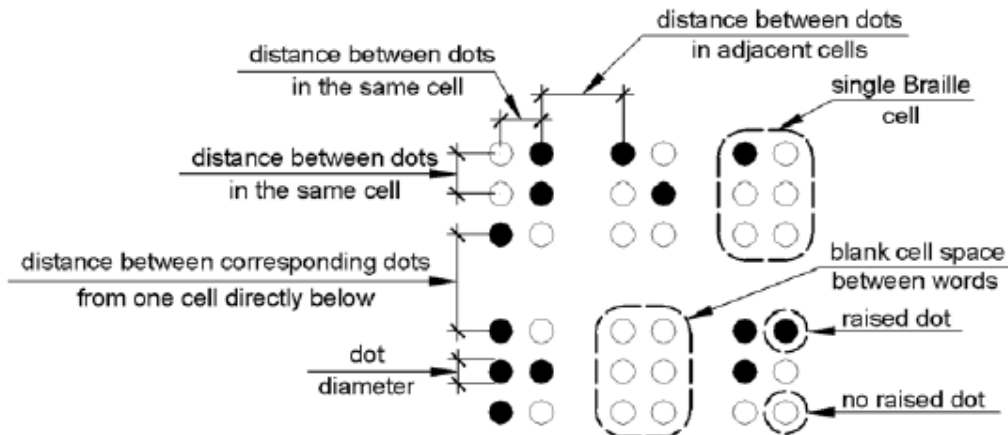
Figure 703.3.1 Braille Measurement
